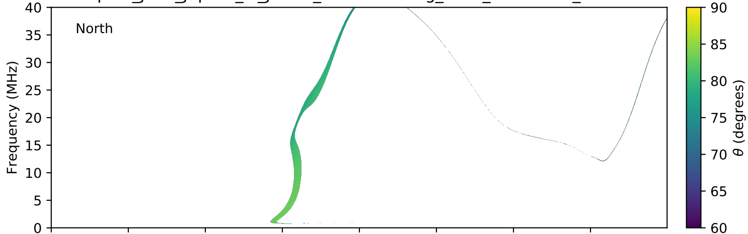
expres_juno_jupiter_io_jrm09_lossc-wid1deg_3kev_20180904_v01.cdf
