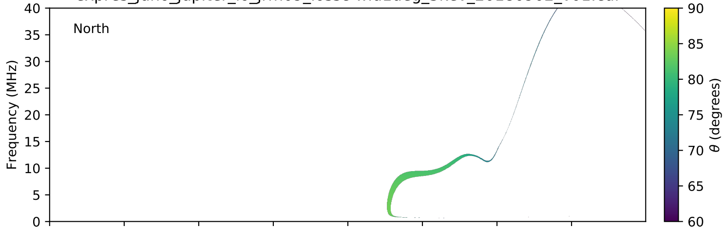
expres_juno_jupiter_io_jrm09_lossc-wid1deg_3kev_20180902_v01.cdf
