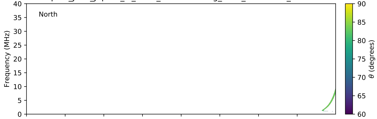
expres_juno_jupiter_io_isaac_lossc-wid1deg_3kev_20180930_v01.cdf
