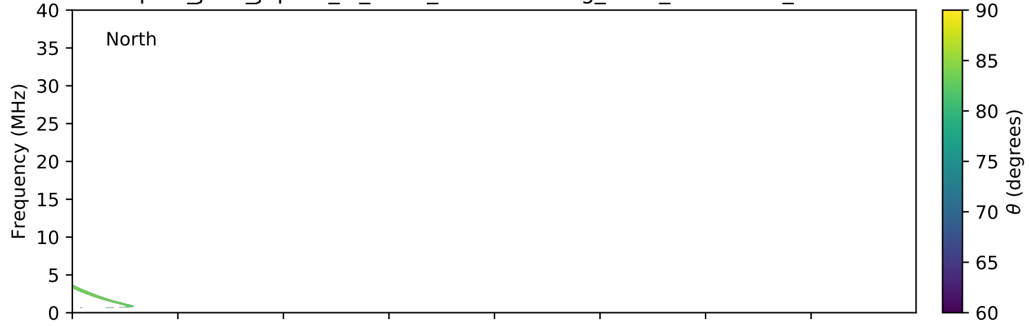
expres_juno_jupiter_io_isaac_lossc-wid1deg_3kev_20180928_v01.cdf
