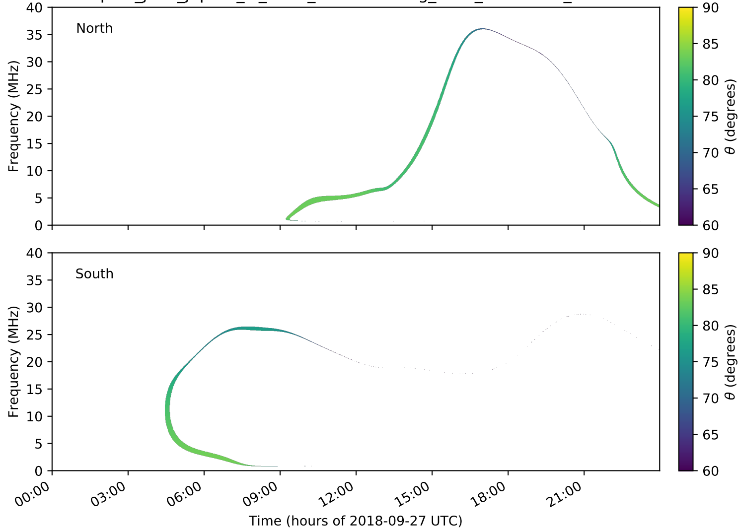
expres_juno_jupiter_io_isaac_lossc-wid1deg_3kev_20180927_v01.cdf
