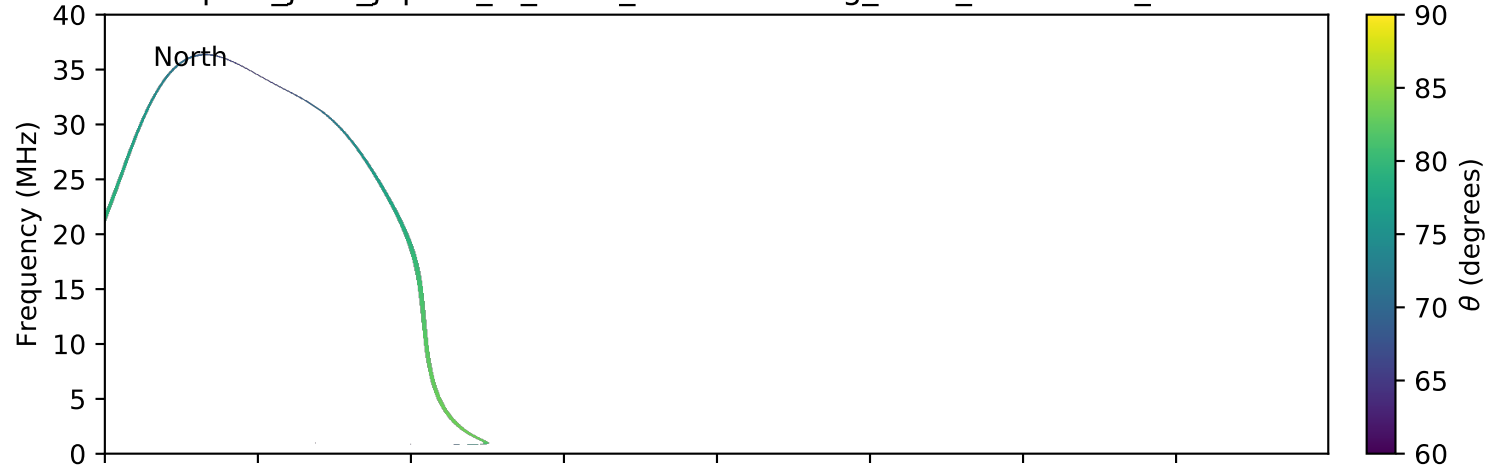
expres_juno_jupiter_io_isaac_lossc-wid1deg_3kev_20180926_v01.cdf
