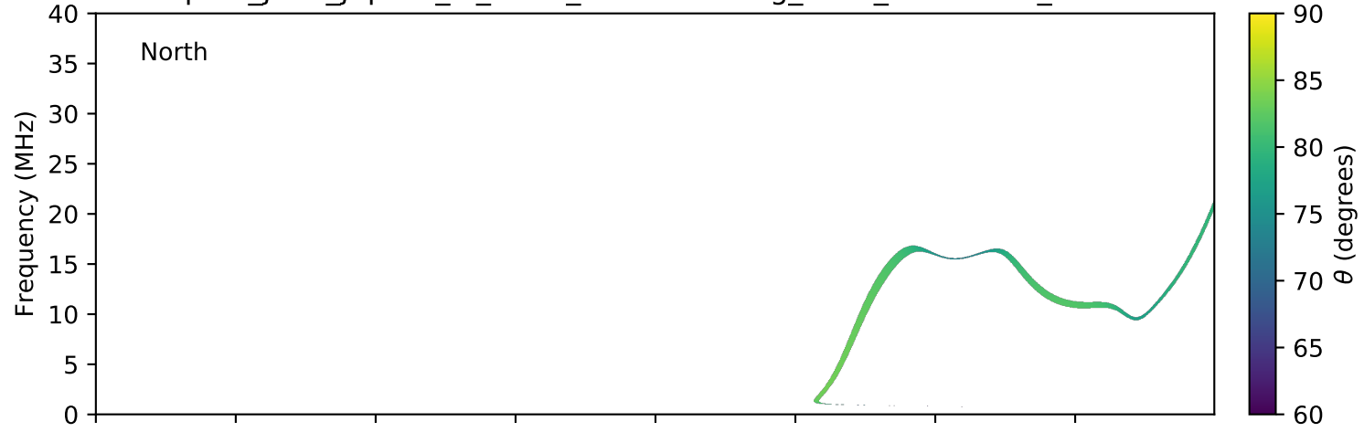
expres_juno_jupiter_io_isaac_lossc-wid1deg_3kev_20180925_v01.cdf
