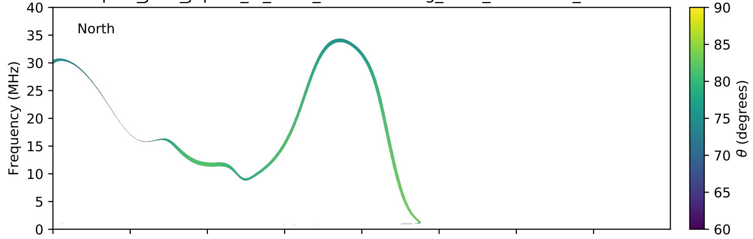
expres_juno_jupiter_io_isaac_lossc-wid1deg_3kev_20180924_v01.cdf
