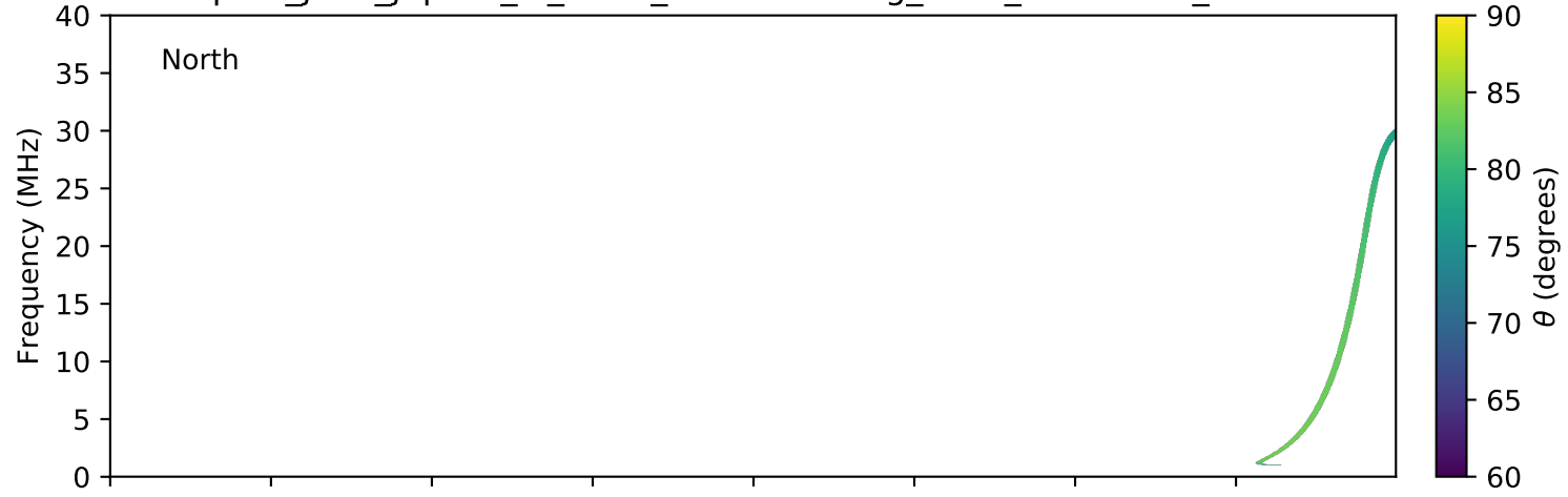
expres_juno_jupiter_io_isaac_lossc-wid1deg_3kev_20180923_v01.cdf
