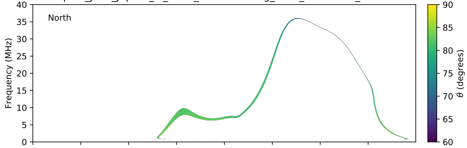
expres_juno_jupiter_io_isaac_lossc-wid1deg_3kev_20180920_v01.cdf
