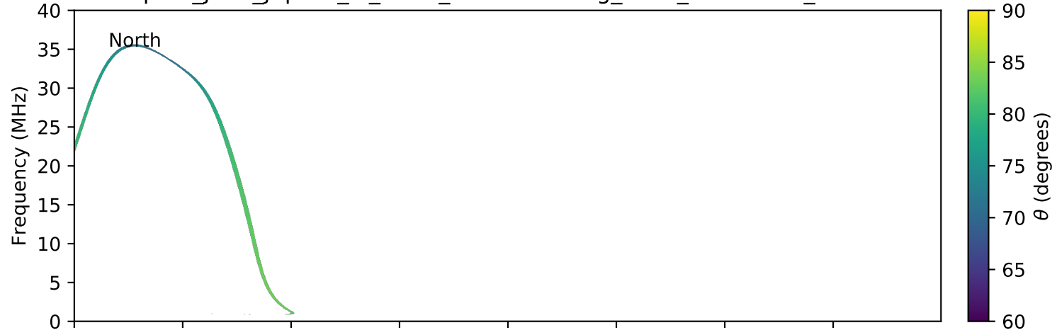
expres_juno_jupiter_io_isaac_lossc-wid1deg_3kev_20180919_v01.cdf
