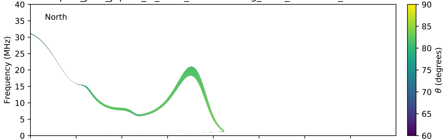
expres_juno_jupiter_io_isaac_lossc-wid1deg_3kev_20180917_v01.cdf
