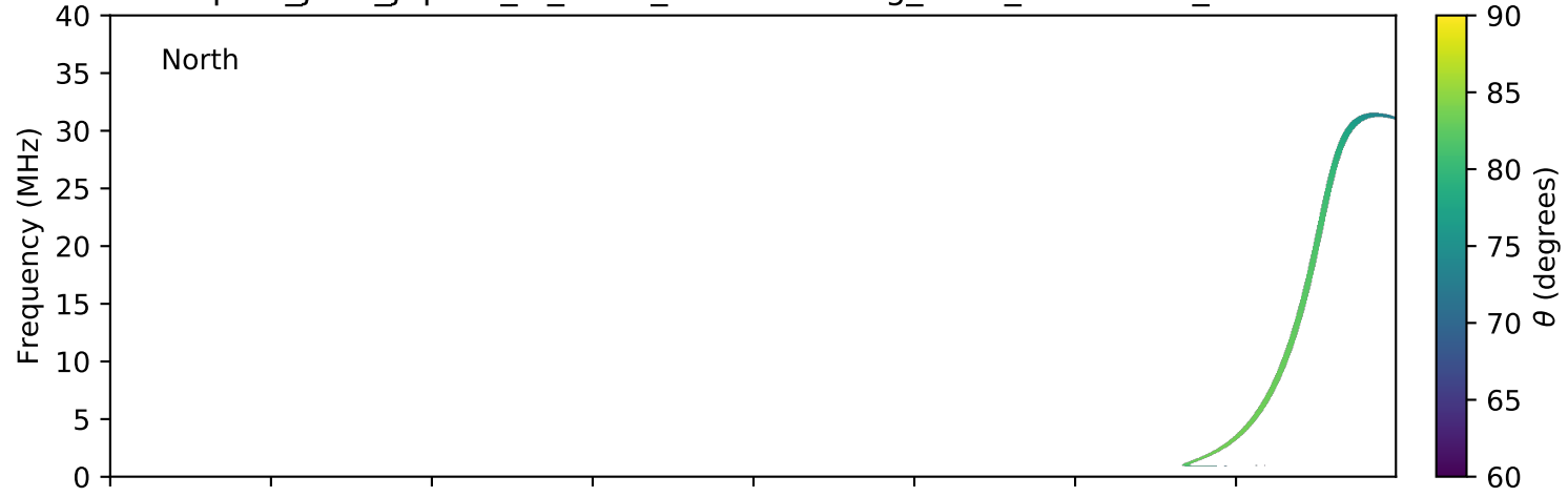
expres_juno_jupiter_io_isaac_lossc-wid1deg_3kev_20180916_v01.cdf
