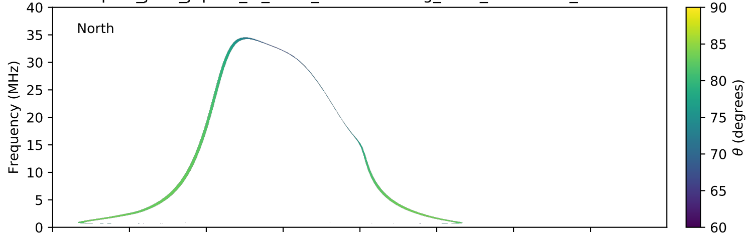
expres_juno_jupiter_io_isaac_lossc-wid1deg_3kev_20180915_v01.cdf
