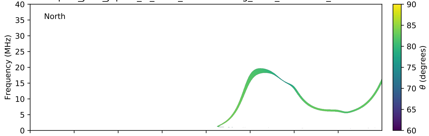
expres_juno_jupiter_io_isaac_lossc-wid1deg_3kev_20180911_v01.cdf
