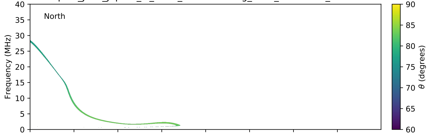
expres_juno_jupiter_io_isaac_lossc-wid1deg_3kev_20180910_v01.cdf
