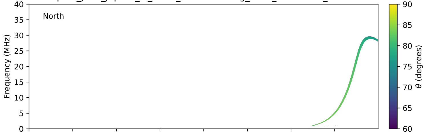
expres_juno_jupiter_io_isaac_lossc-wid1deg_3kev_20180909_v01.cdf
