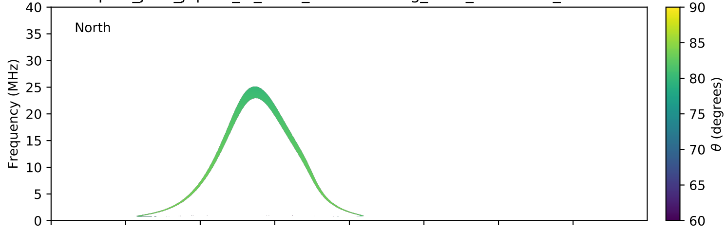
expres_juno_jupiter_io_isaac_lossc-wid1deg_3kev_20180908_v01.cdf
