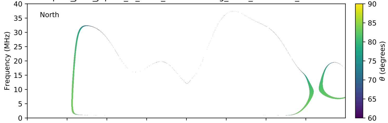
expres_juno_jupiter_io_isaac_lossc-wid1deg_3kev_20180906_v01.cdf
