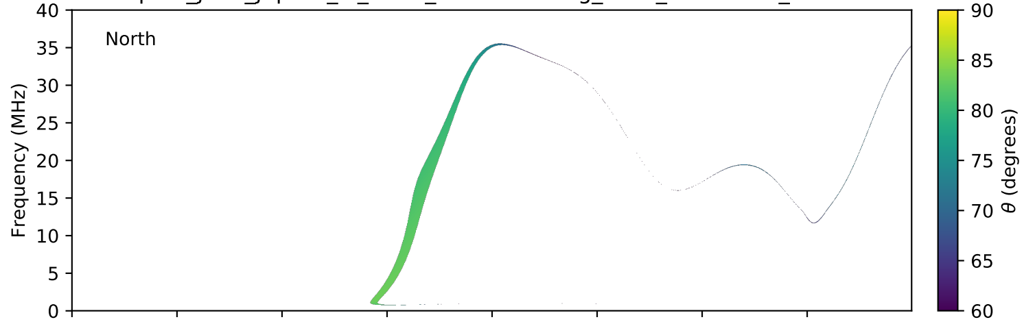
expres_juno_jupiter_io_isaac_lossc-wid1deg_3kev_20180904_v01.cdf
