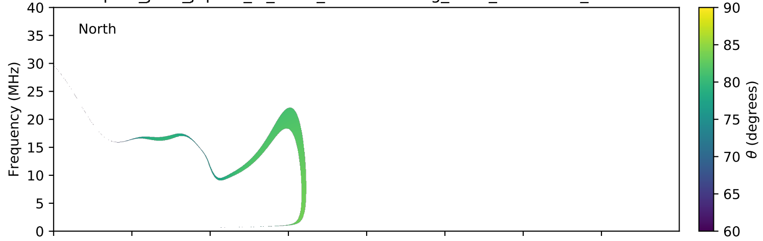
expres_juno_jupiter_io_isaac_lossc-wid1deg_3kev_20180903_v01.cdf
