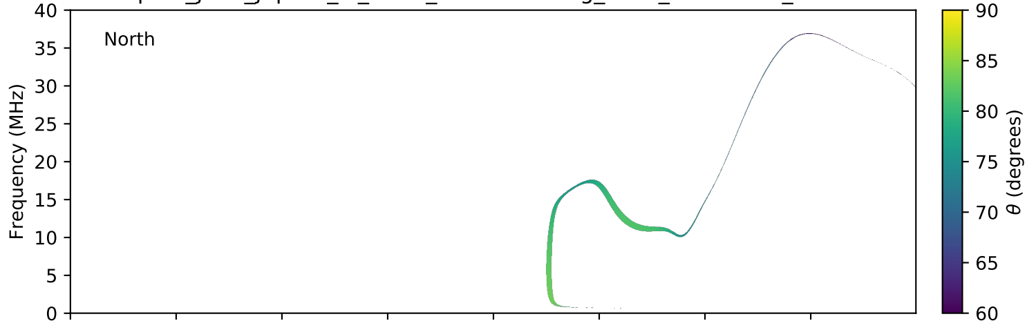
expres_juno_jupiter_io_isaac_lossc-wid1deg_3kev_20180902_v01.cdf
