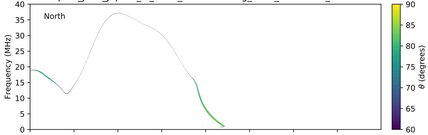
expres_juno_jupiter_io_isaac_lossc-wid1deg_3kev_20180901_v01.cdf
