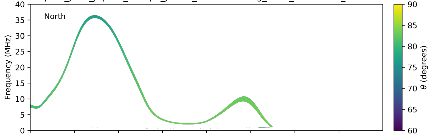
expres_juno_jupiter_europa_jrm09_lossc-wid1deg_3kev_20180928_v01.cdf
