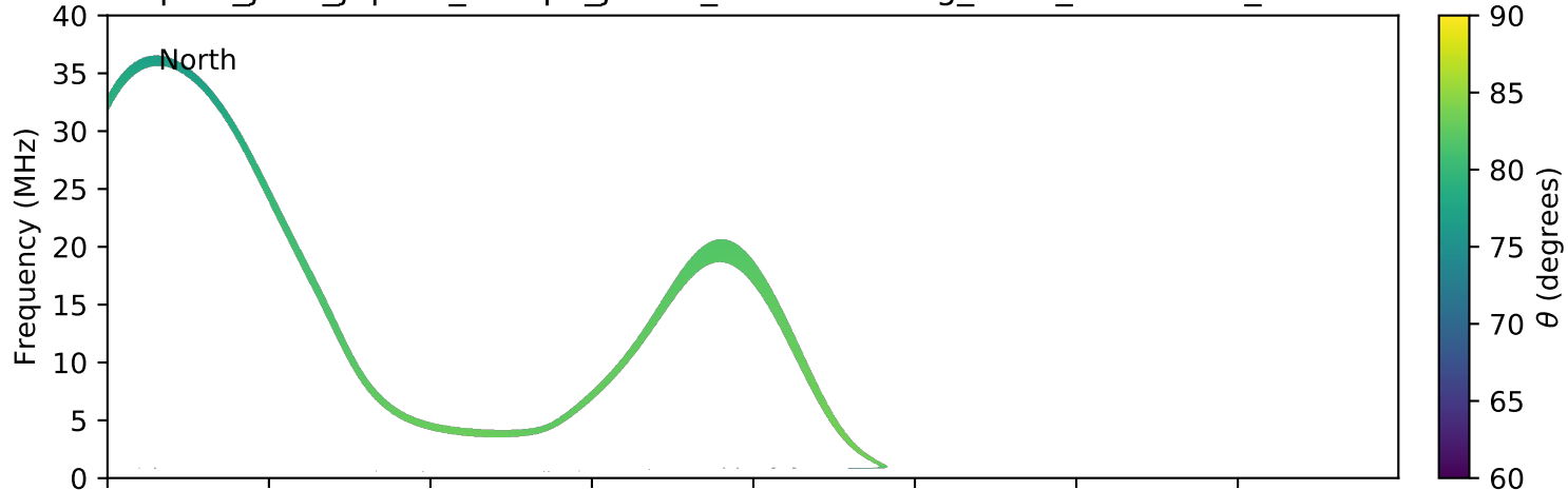
expres_juno_jupiter_europa_jrm09_lossc-wid1deg_3kev_20180924_v01.cdf
