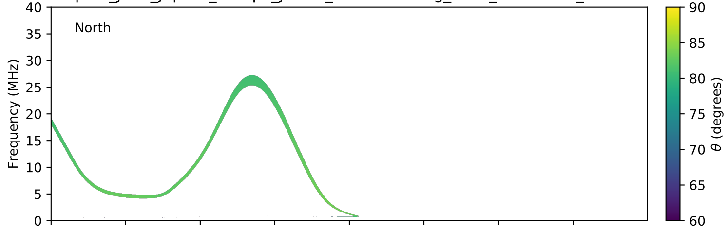
expres_juno_jupiter_europa_jrm09_lossc-wid1deg_3kev_20180920_v01.cdf
