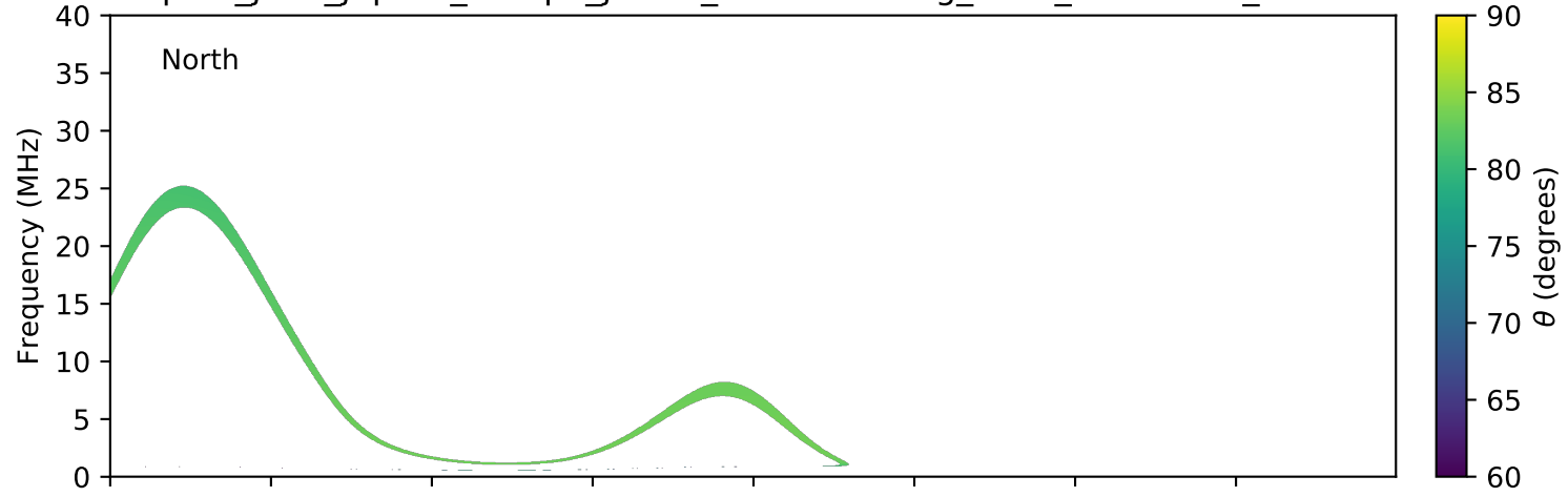
expres_juno_jupiter_europa_jrm09_lossc-wid1deg_3kev_20180912_v01.cdf
