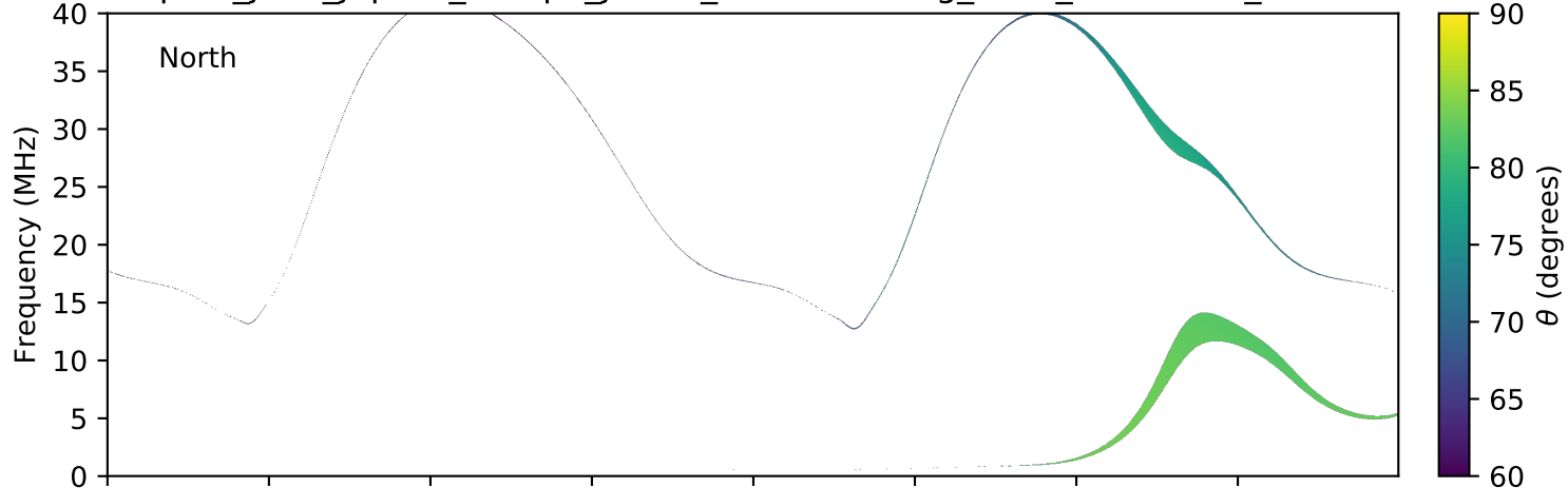
expres_juno_jupiter_europa_jrm09_lossc-wid1deg_3kev_20180906_v01.cdf
