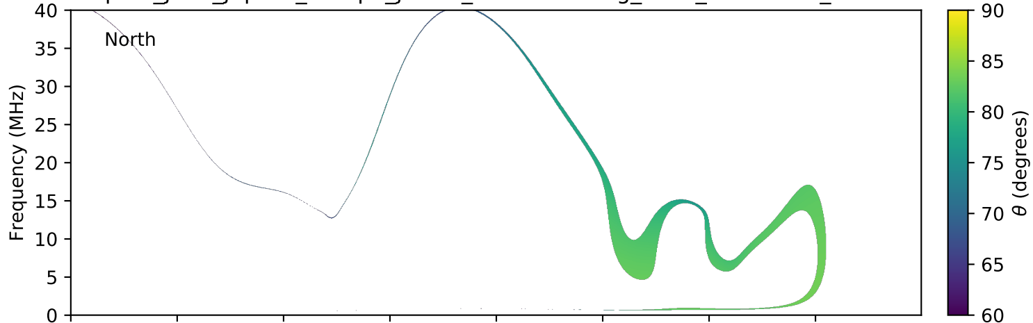
expres_juno_jupiter_europa_jrm09_lossc-wid1deg_3kev_20180905_v01.cdf
