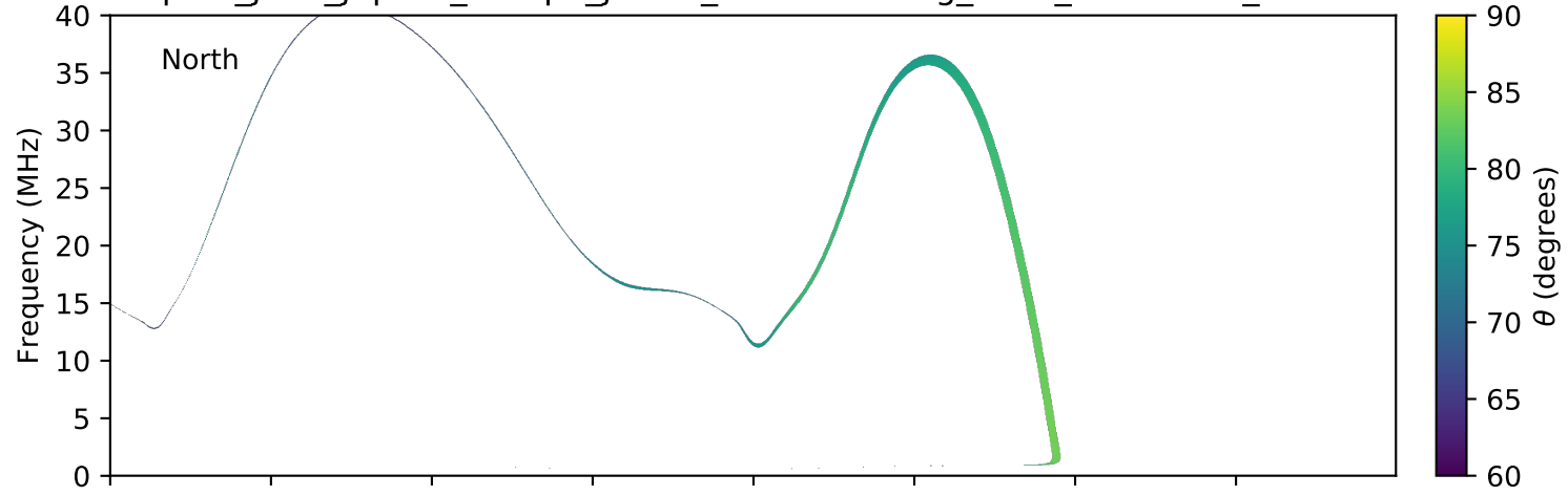
expres_juno_jupiter_europa_jrm09_lossc-wid1deg_3kev_20180904_v01.cdf
