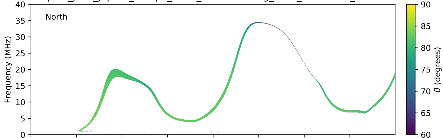
expres_juno_jupiter_europa_isaac_lossc-wid1deg_3kev_20180930_v01.cdf
