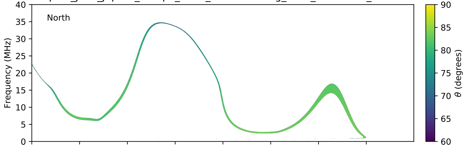
expres_juno_jupiter_europa_isaac_lossc-wid1deg_3kev_20180927_v01.cdf
