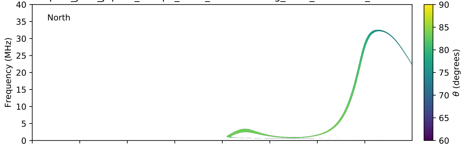
expres_juno_jupiter_europa_isaac_lossc-wid1deg_3kev_20180926_v01.cdf
