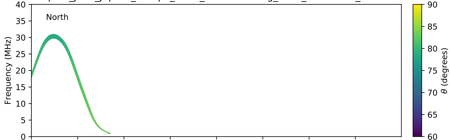
expres_juno_jupiter_europa_isaac_lossc-wid1deg_3kev_20180924_v01.cdf
