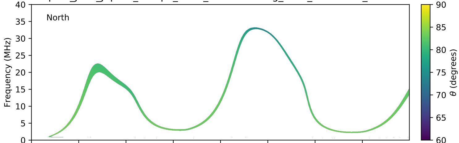
expres_juno_jupiter_europa_isaac_lossc-wid1deg_3kev_20180916_v01.cdf
