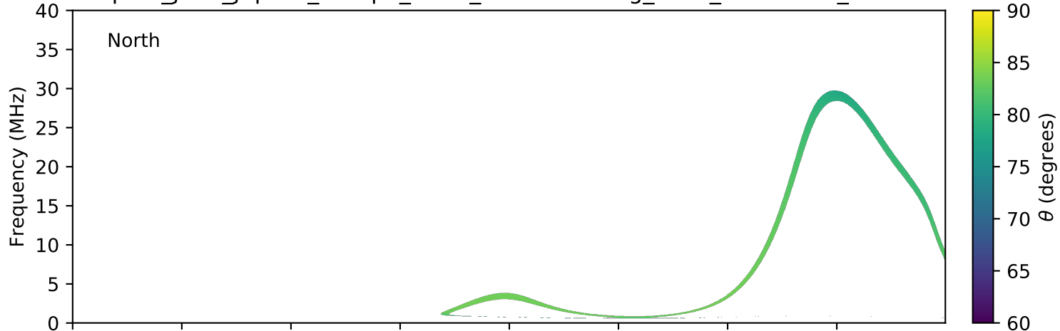
expres_juno_jupiter_europa_isaac_lossc-wid1deg_3kev_20180912_v01.cdf
