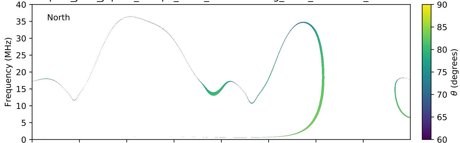
expres_juno_jupiter_europa_isaac_lossc-wid1deg_3kev_20180906_v01.cdf
