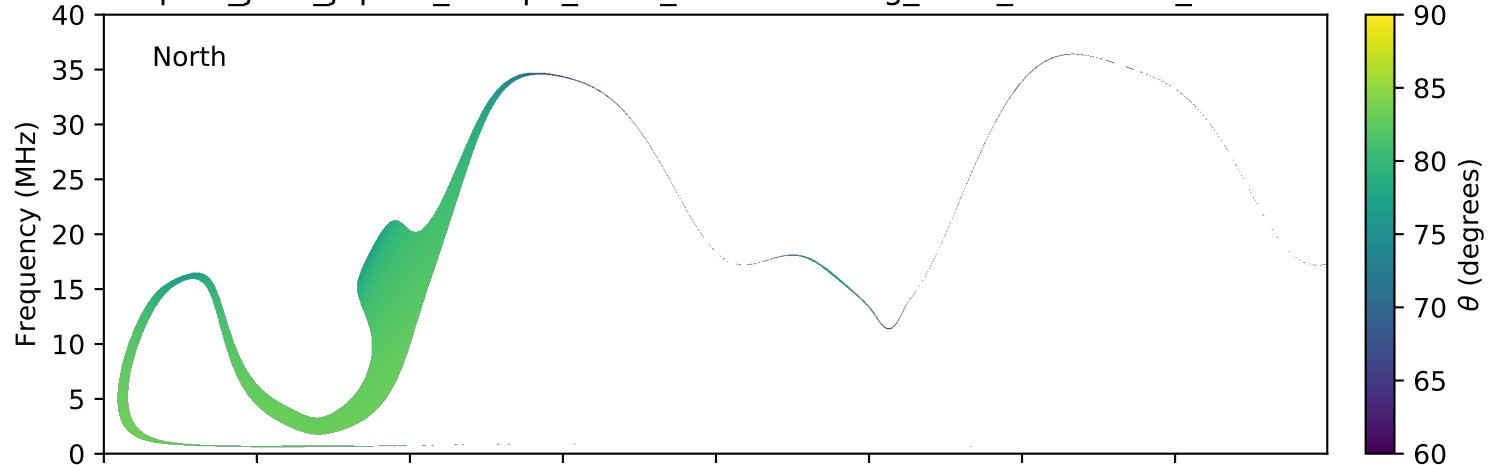
expres_juno_jupiter_europa_isaac_lossc-wid1deg_3kev_20180905_v01.cdf
