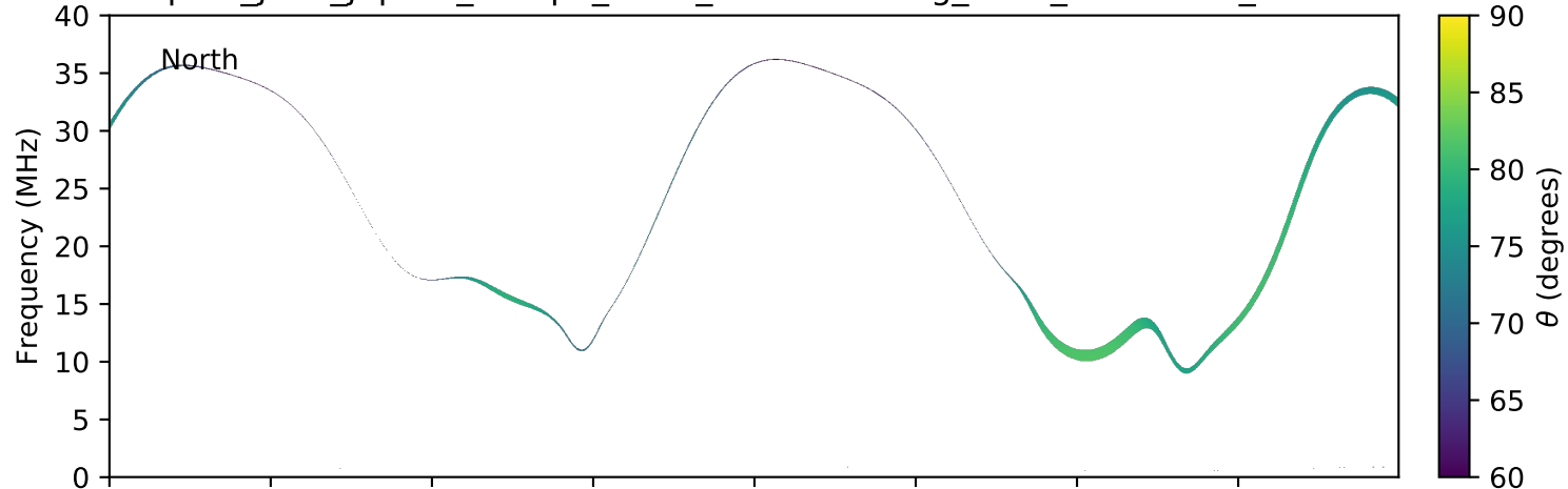
expres_juno_jupiter_europa_isaac_lossc-wid1deg_3kev_20180902_v01.cdf
