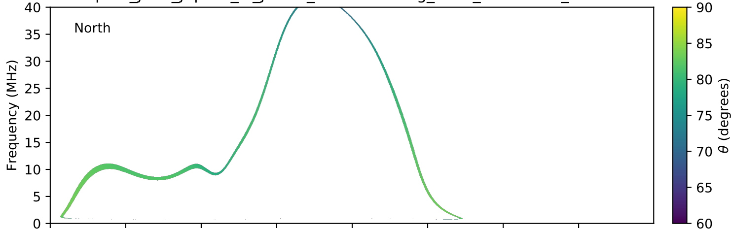
expres_juno_jupiter_io_jrm09_lossc-wid1deg_3kev_20180731_v01.cdf
