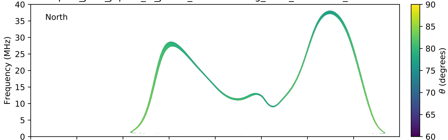
expres_juno_jupiter_io_jrm09_lossc-wid1deg_3kev_20180729_v01.cdf
