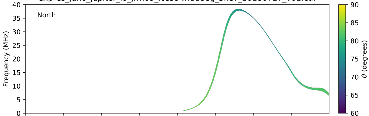
expres_juno_jupiter_io_jrm09_lossc-wid1deg_3kev_20180727_v01.cdf
