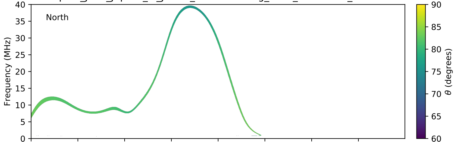
expres_juno_jupiter_io_jrm09_lossc-wid1deg_3kev_20180724_v01.cdf
