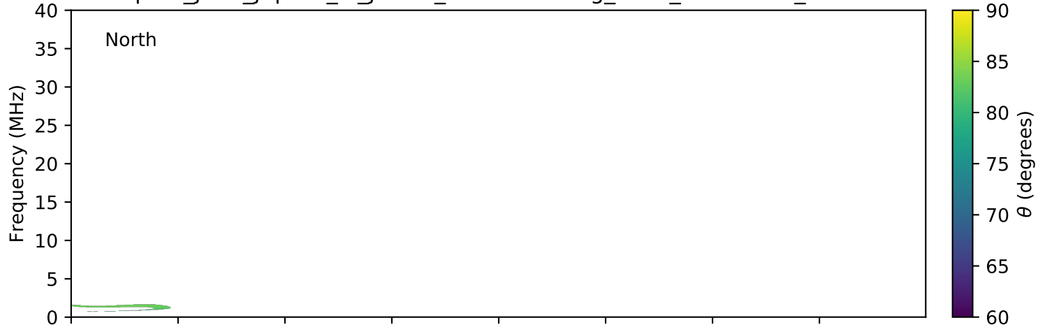
expres_juno_jupiter_io_jrm09_lossc-wid1deg_3kev_20180721_v01.cdf
