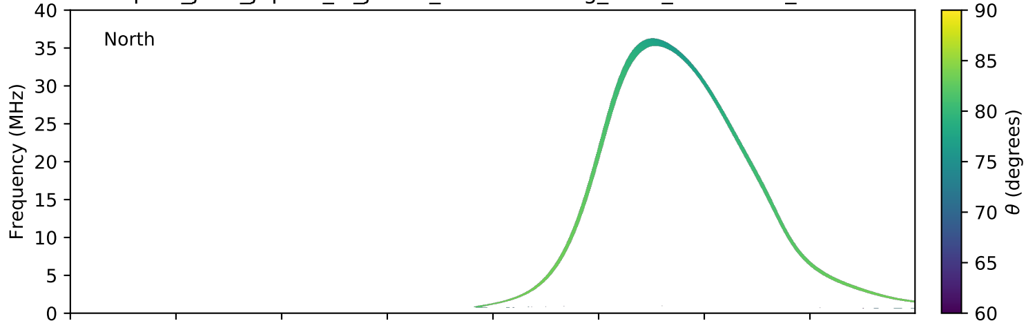
expres_juno_jupiter_io_jrm09_lossc-wid1deg_3kev_20180720_v01.cdf
