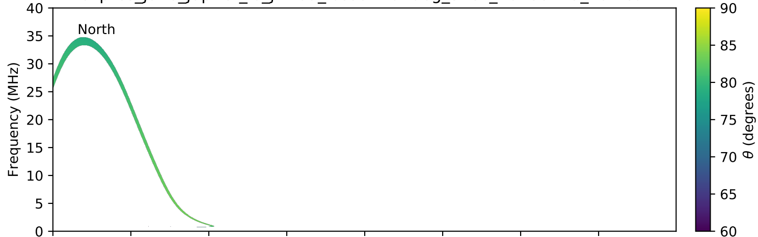
expres_juno_jupiter_io_jrm09_lossc-wid1deg_3kev_20180719_v01.cdf
