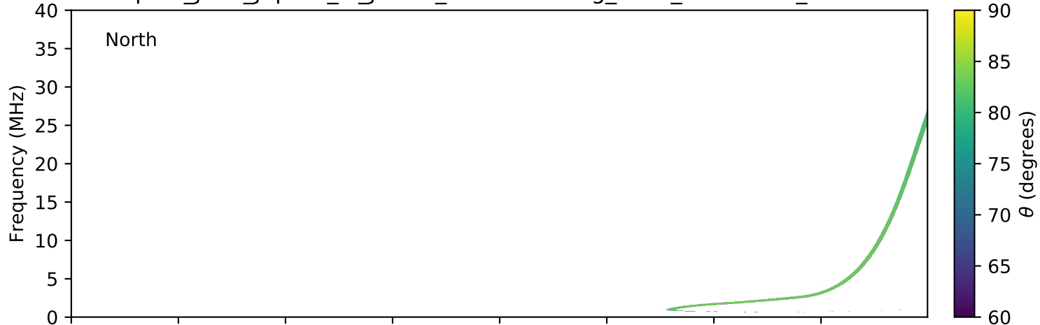
expres_juno_jupiter_io_jrm09_lossc-wid1deg_3kev_20180718_v01.cdf
