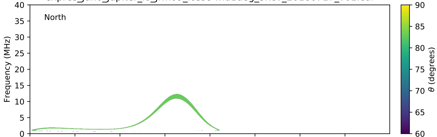
expres_juno_jupiter_io_jrm09_lossc-wid1deg_3kev_20180717_v01.cdf
