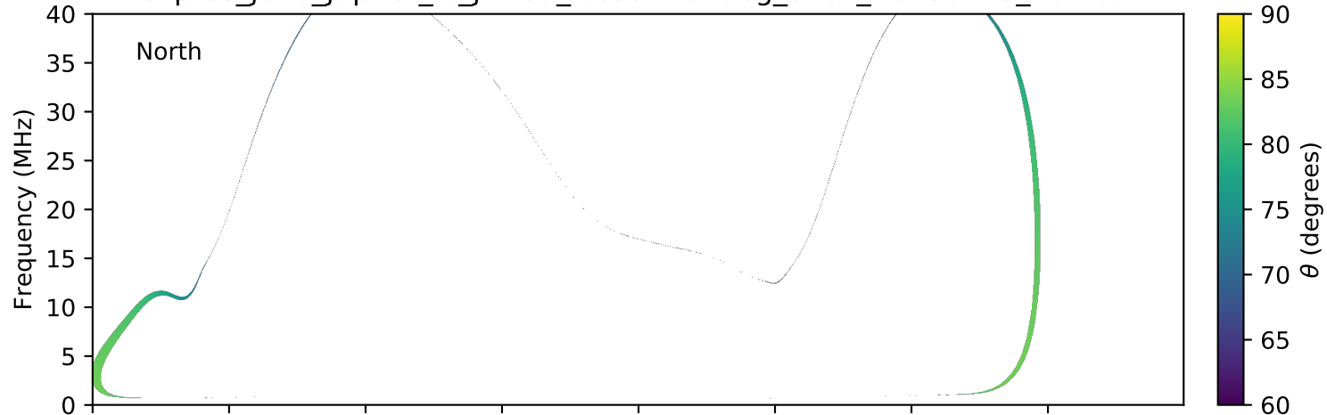
expres_juno_jupiter_io_jrm09_lossc-wid1deg_3kev_20180715_v01.cdf
