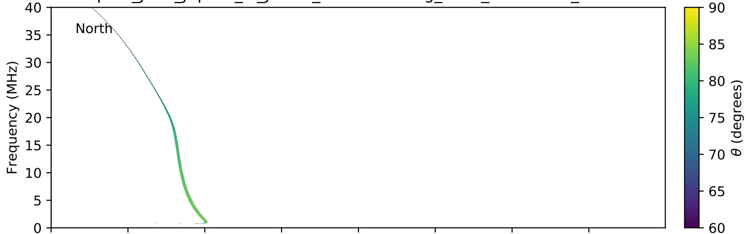
expres_juno_jupiter_io_jrm09_lossc-wid1deg_3kev_20180712_v01.cdf
